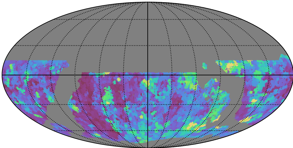
noroll_mjdp0_v3.4_10yrs WFD g band: Max seeingEff
