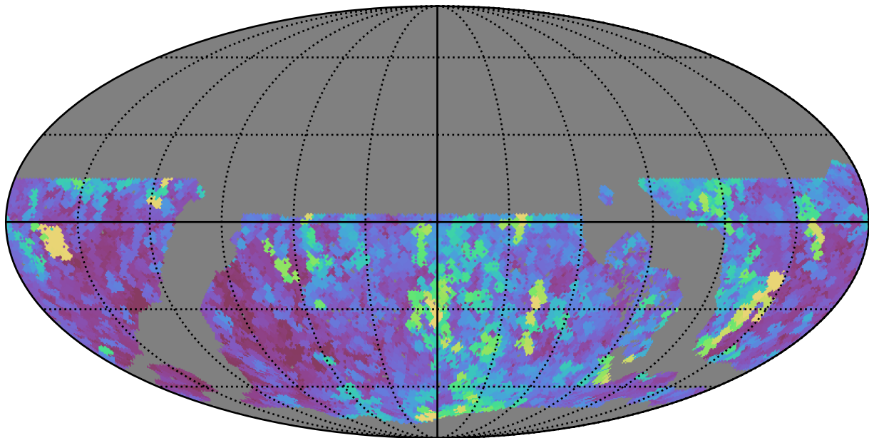
noroll_mjdp0_v3.4_10yrs WFD all bands: Max seeingEff
