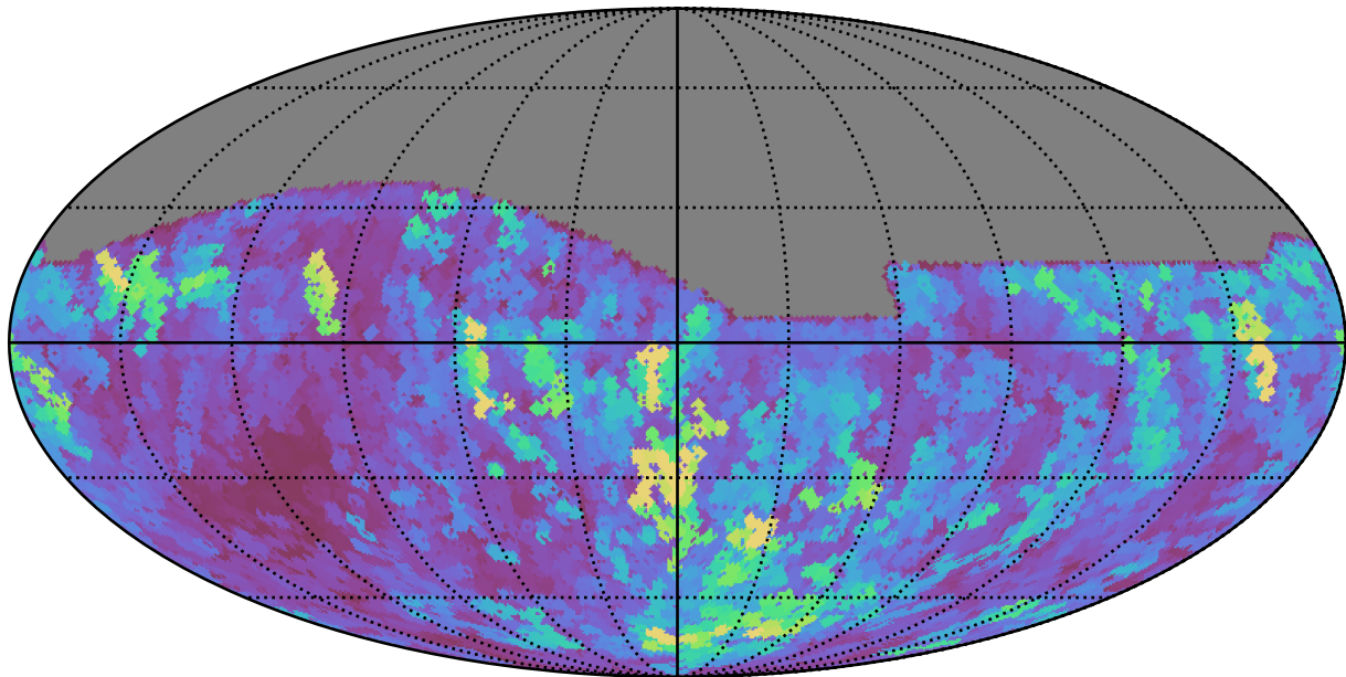
noroll_mjdp0_v3.4_10yrs All sky z band: Max seeingEff
