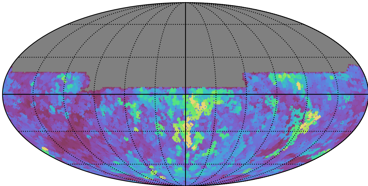
noroll_mjdp0_v3.4_10yrs All sky y band: Max seeingEff
