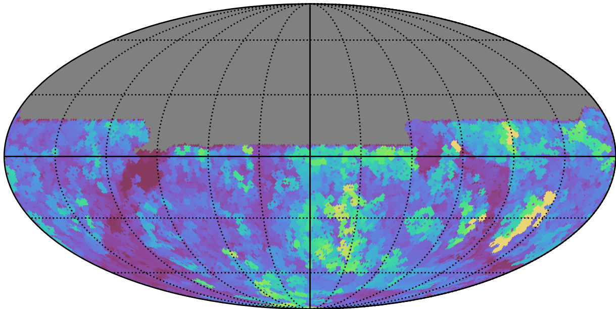
noroll_mjdp0_v3.4_10yrs All sky u band: Max seeingEff
