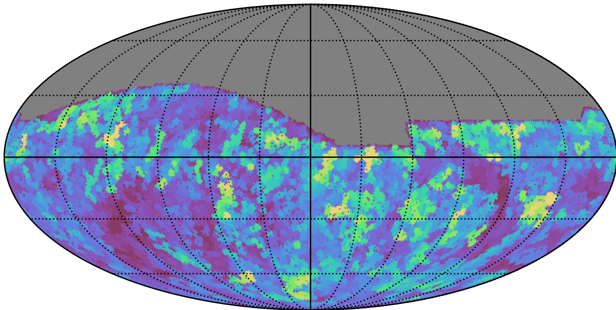
noroll_mjdp0_v3.4_10yrs All sky r band: Max seeingEff
