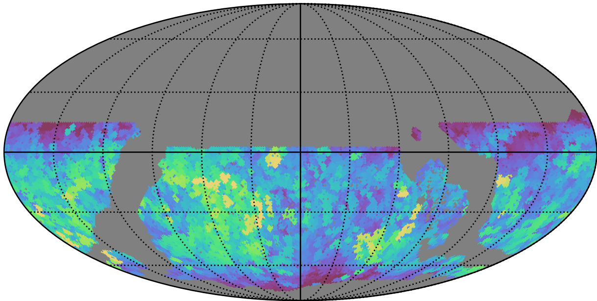
noroll_mjdp0_v3.4_10yrs WFD i band: Max saturation_mag
