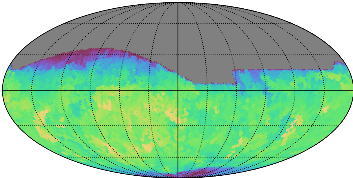
noroll_mjdp0_v3.4_10yrs All sky r band: Max saturation_mag
