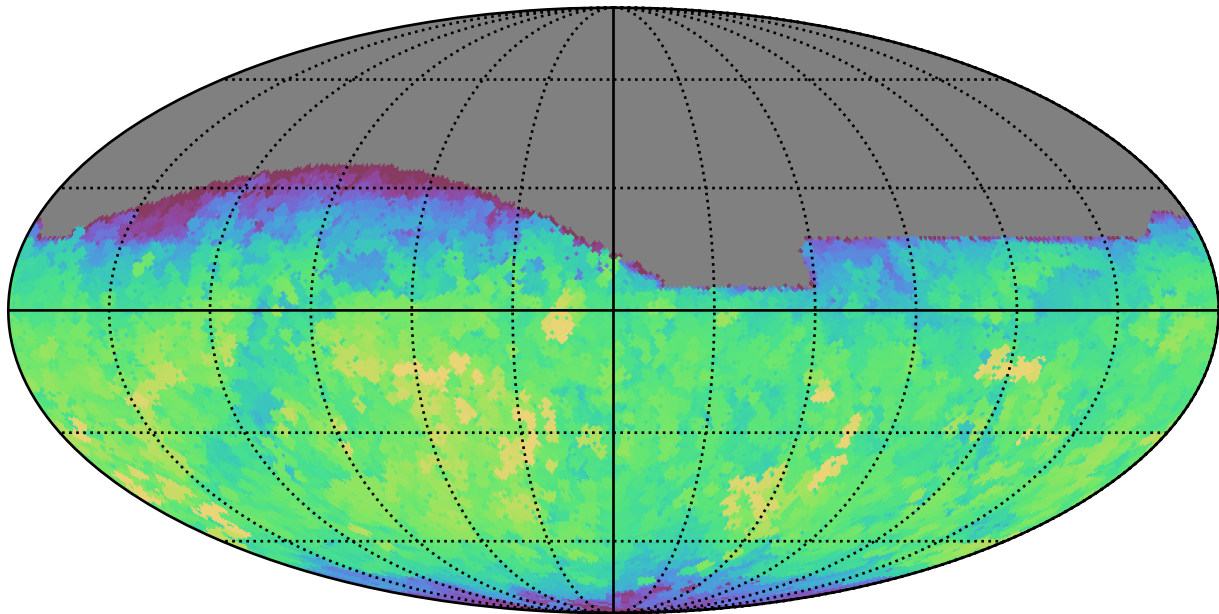
noroll_mjdp0_v3.4_10yrs All sky i band: Max saturation_mag
