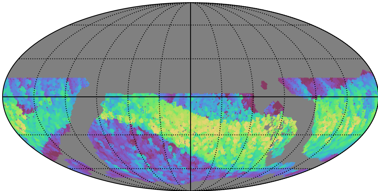
noroll_mjdp0_v3.4_10yrs WFD z band: Max normairmass
