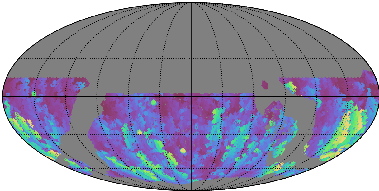
noroll_mjdp0_v3.4_10yrs WFD u band: Max normairmass
