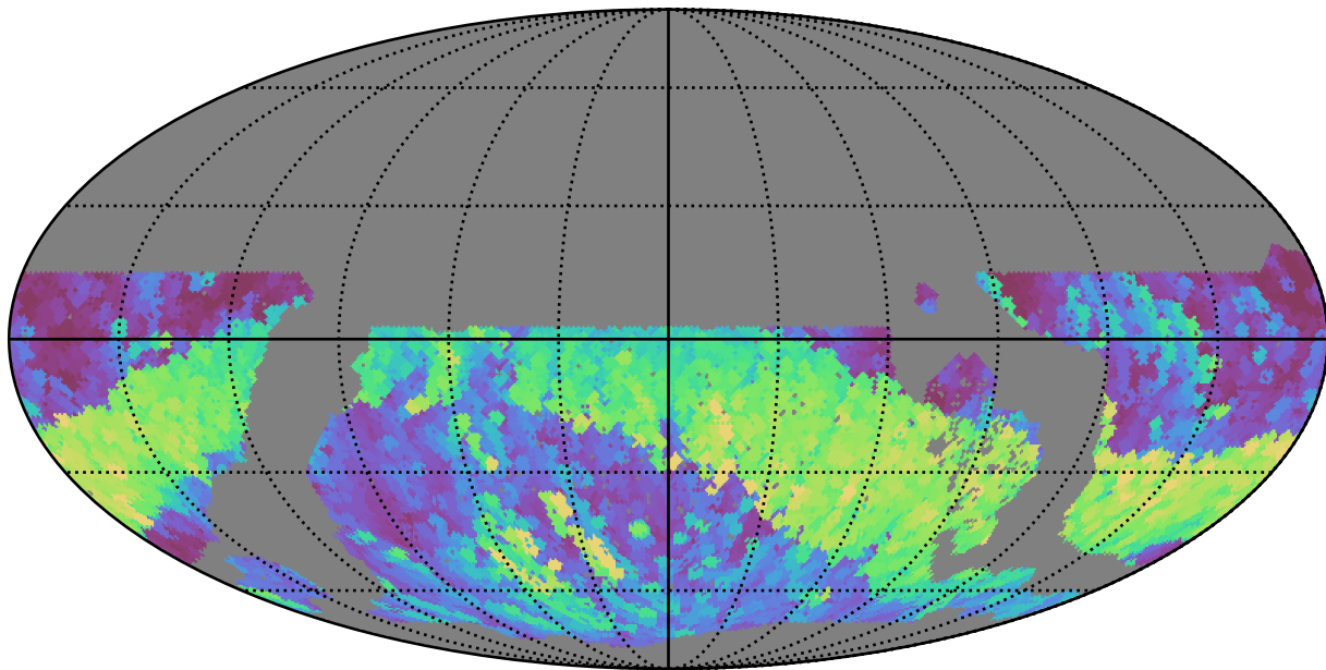
noroll_mjdp0_v3.4_10yrs WFD r band: Max normairmass
