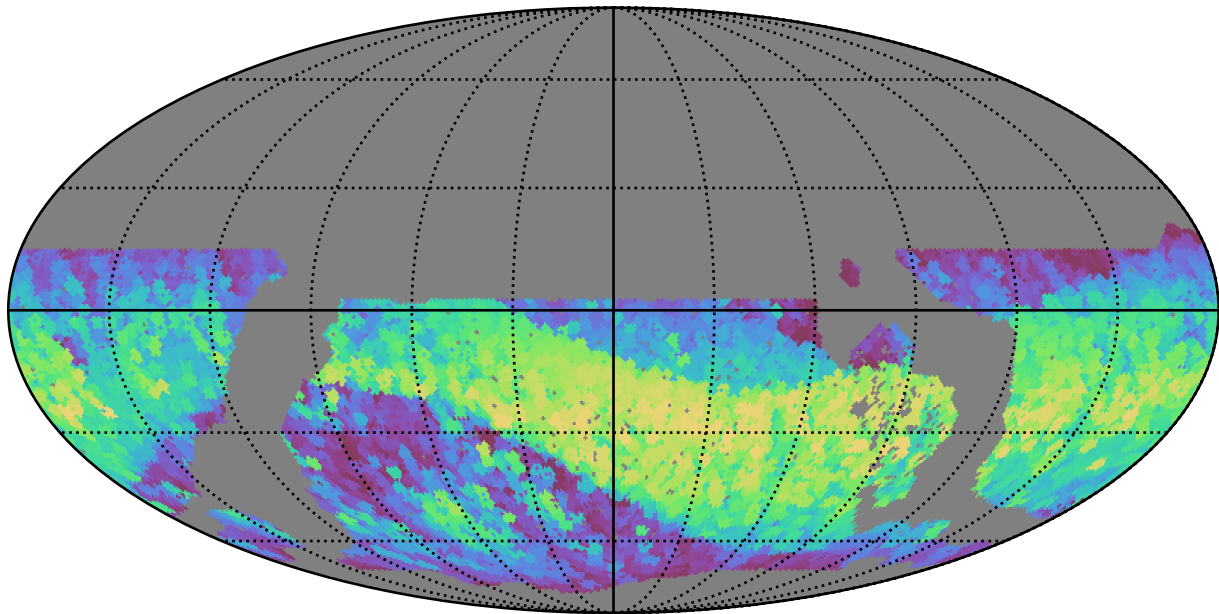
noroll_mjdp0_v3.4_10yrs WFD all bands: Max normairmass
