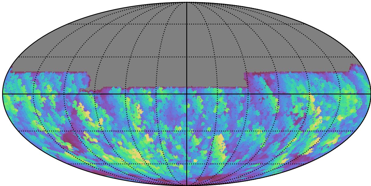
noroll_mjdp0_v3.4_10yrs All sky y band: Max normairmass
