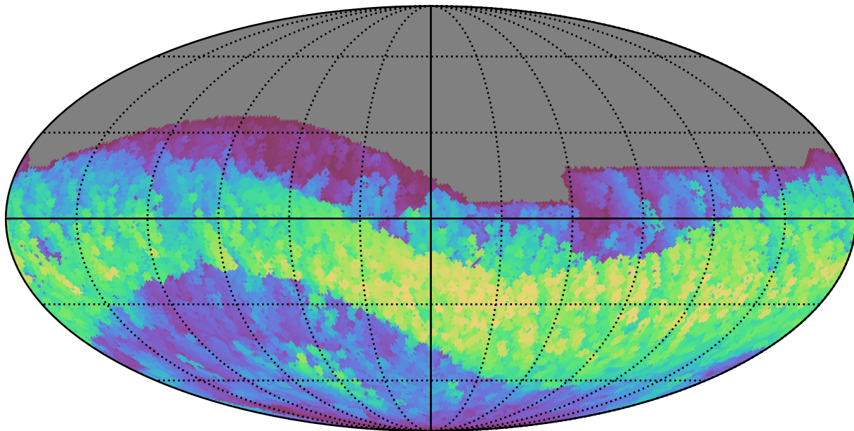
noroll_mjdp0_v3.4_10yrs All sky i band: Max normairmass
