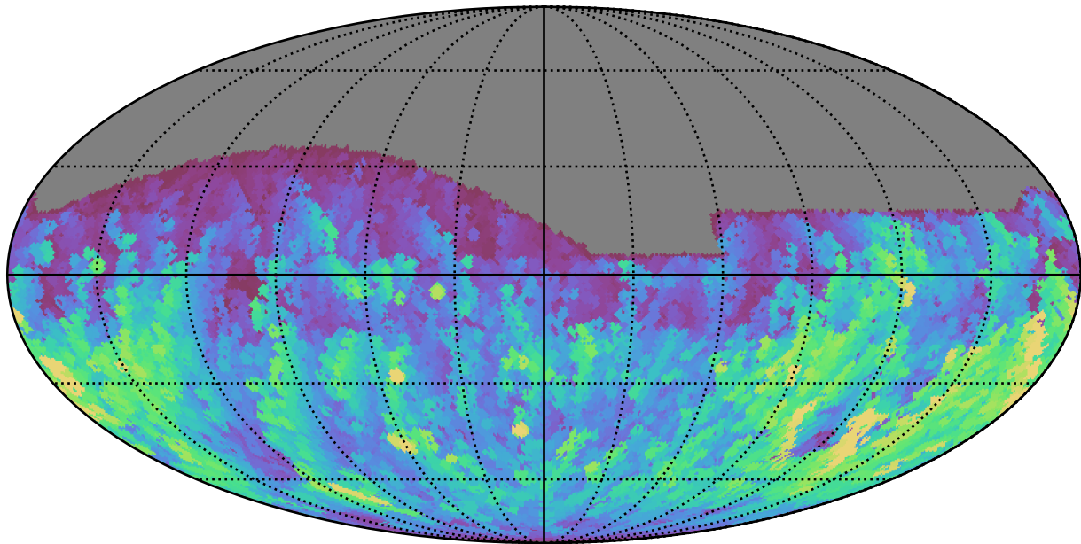
noroll_mjdp0_v3.4_10yrs All sky g band: Max normairmass
