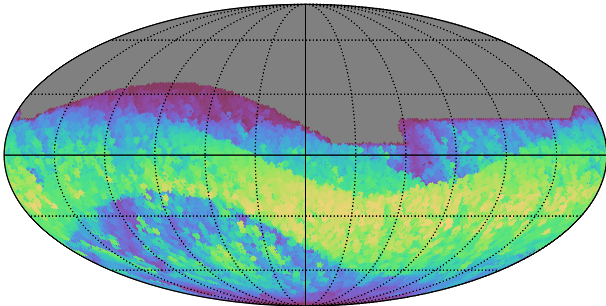
noroll_mjdp0_v3.4_10yrs All sky all bands: Max normairmass
