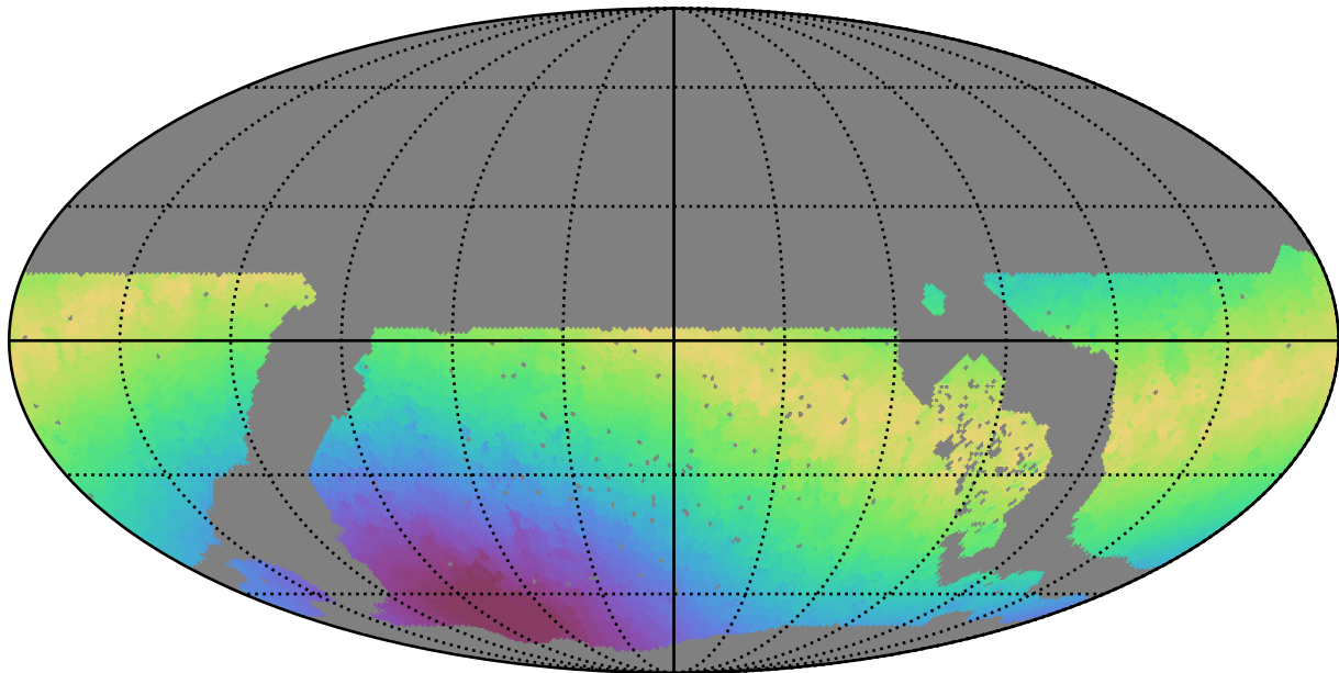
noroll_mjdp0_v3.4_10yrs WFD z band: Max moonDistance
