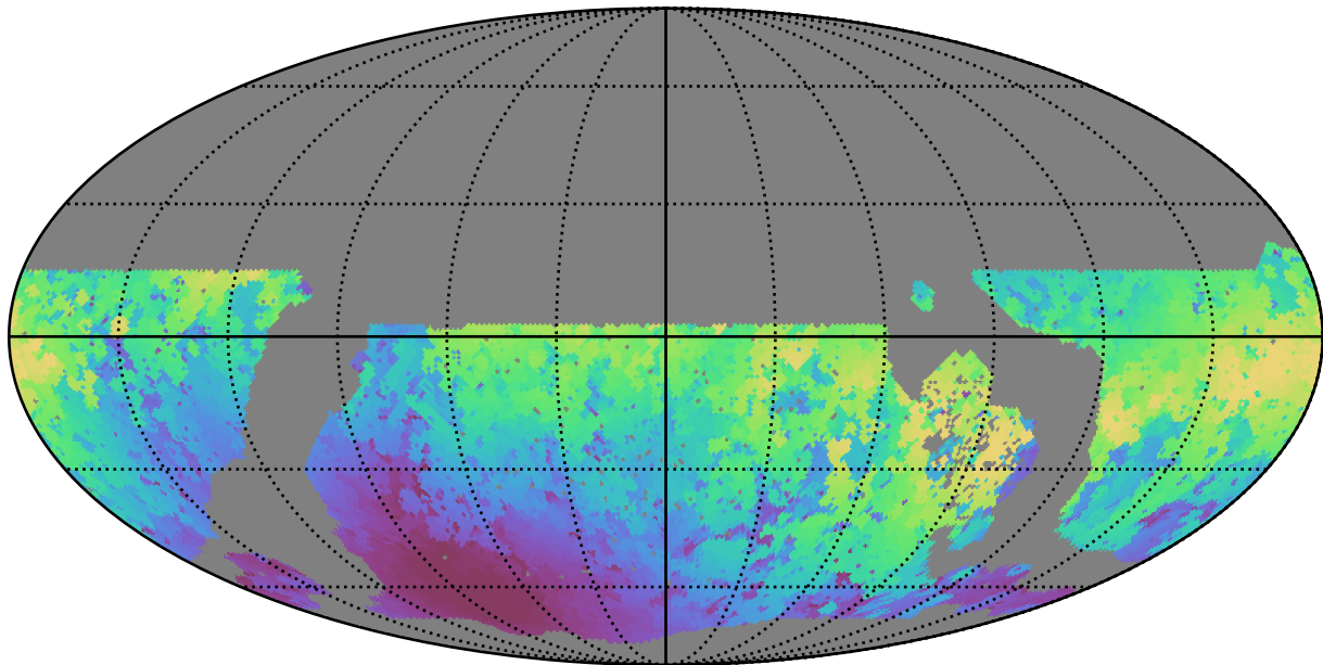
noroll_mjdp0_v3.4_10yrs WFD y band: Max moonDistance
