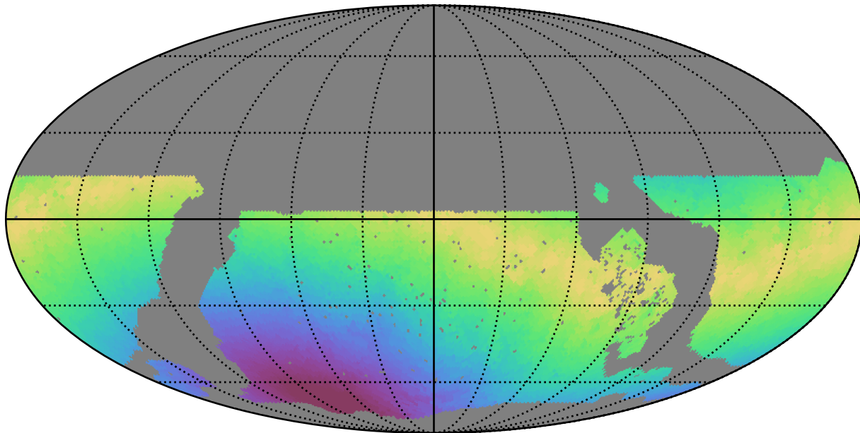
noroll_mjdp0_v3.4_10yrs WFD u band: Max moonDistance
