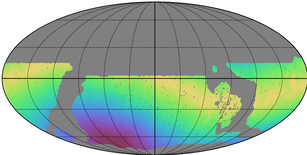
noroll_mjdp0_v3.4_10yrs WFD g band: Max moonDistance
