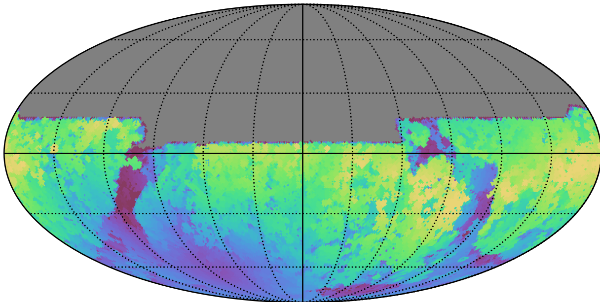
noroll_mjdp0_v3.4_10yrs All sky y band: Max moonDistance
