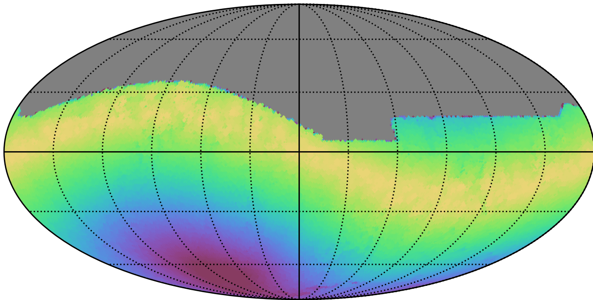
noroll_mjdp0_v3.4_10yrs All sky r band: Max moonDistance
