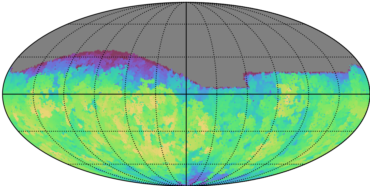
noroll_mjdp0_v3.4_10yrs Yr 1 all bands: Max fiveSigmaDepth
