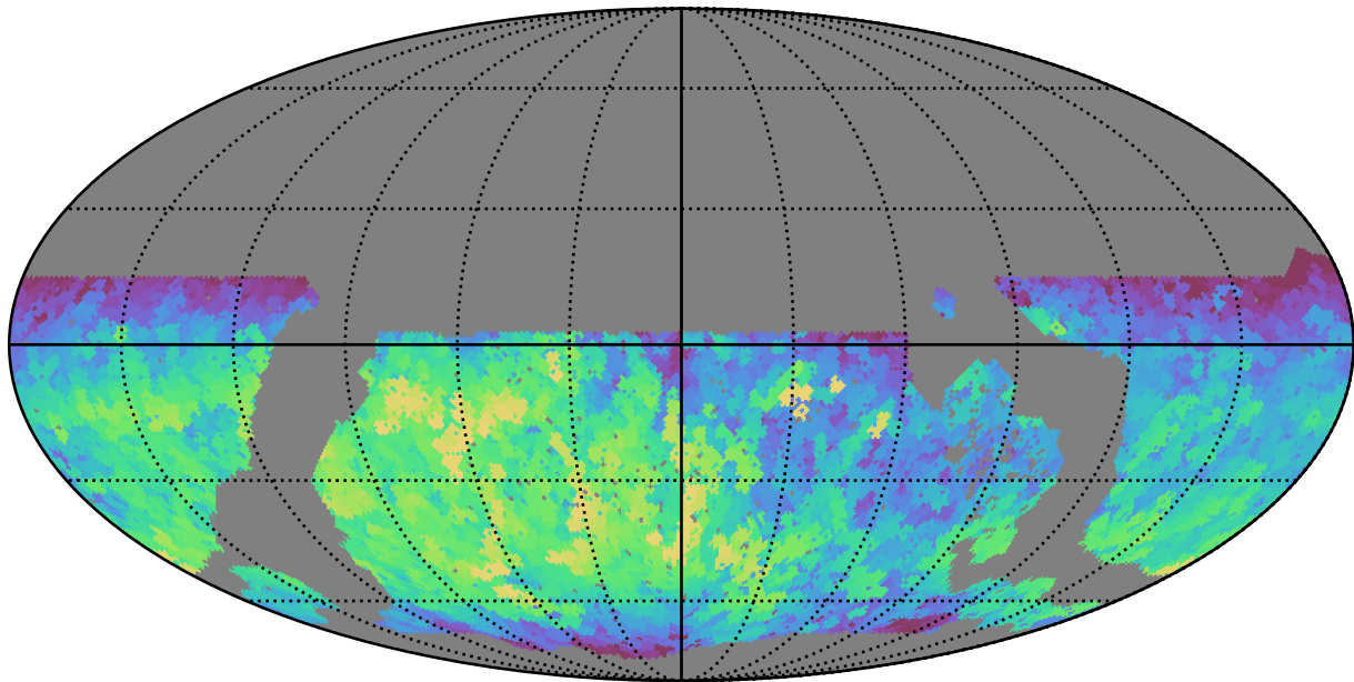
noroll_mjdp0_v3.4_10yrs WFD all bands: Max fiveSigmaDepth
