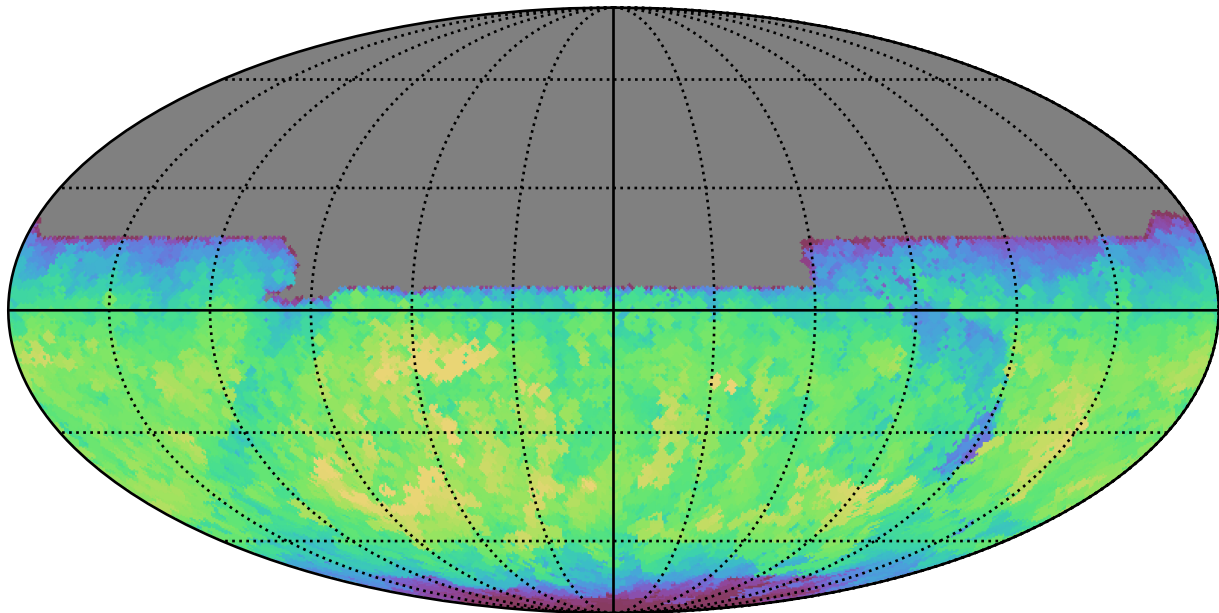
noroll_mjdp0_v3.4_10yrs All sky y band: Max fiveSigmaDepth
