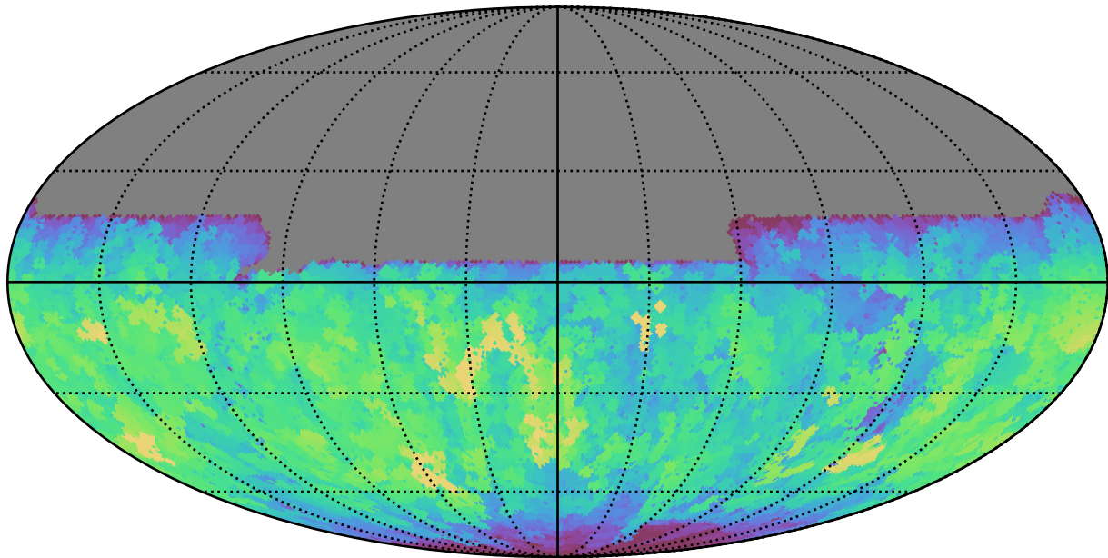
noroll_mjdp0_v3.4_10yrs All sky u band: Max fiveSigmaDepth
