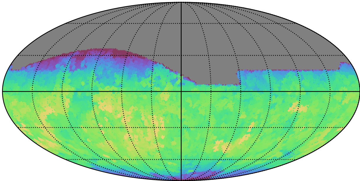
noroll_mjdp0_v3.4_10yrs All sky i band: Max fiveSigmaDepth
