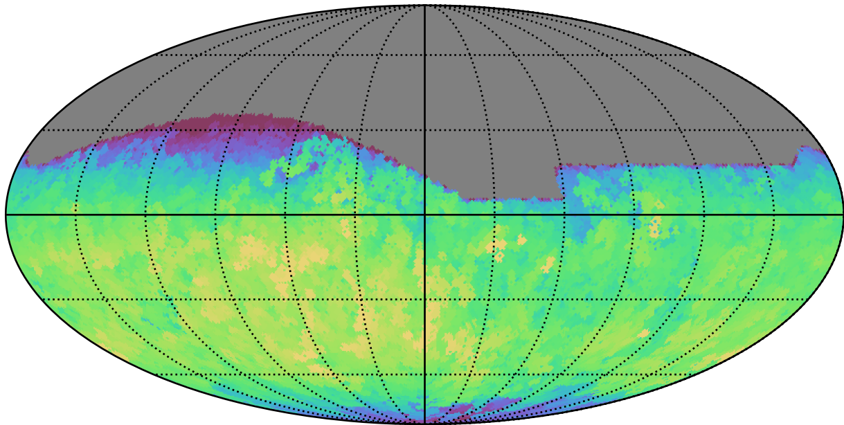
noroll_mjdp0_v3.4_10yrs All sky g band: Max fiveSigmaDepth
