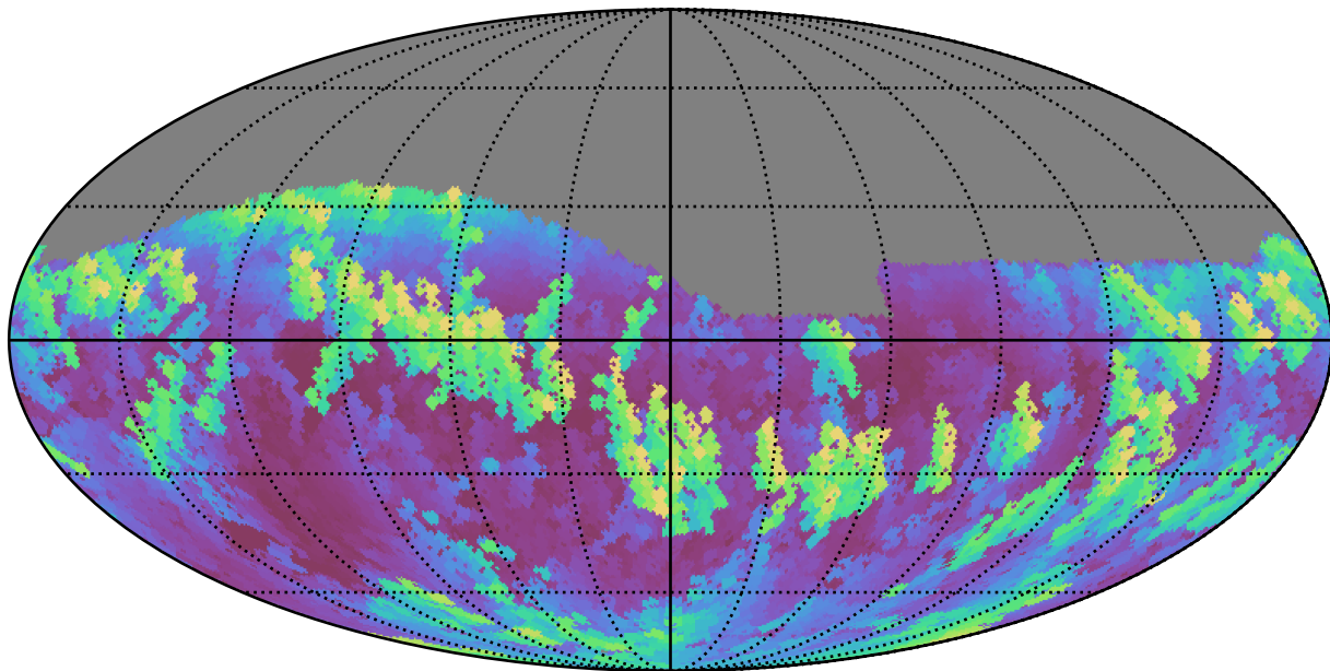
noroll_mjdp0_v3.4_10yrs Yr 1 z band: Max airmass
