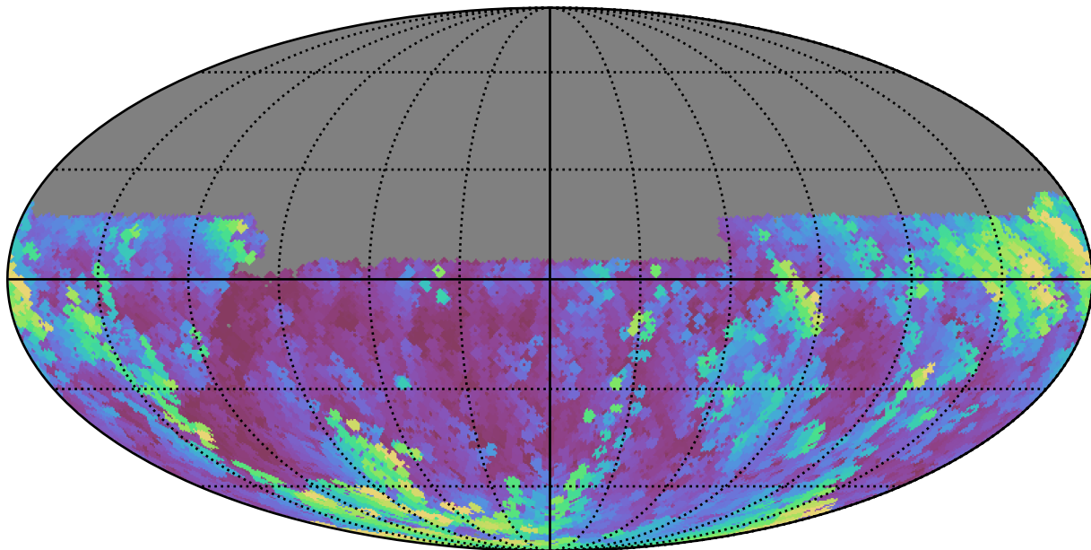
noroll_mjdp0_v3.4_10yrs Yr 1 y band: Max airmass
