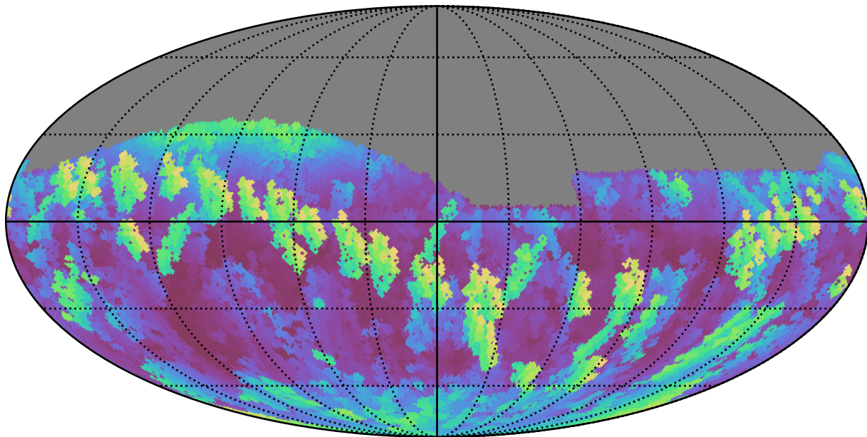
noroll_mjdp0_v3.4_10yrs Yr 1 i band: Max airmass
