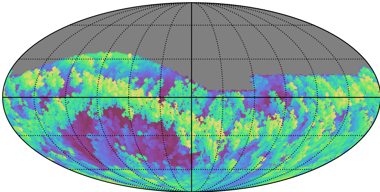
noroll_mjdp0_v3.4_10yrs Yr 1 all bands: Max airmass
