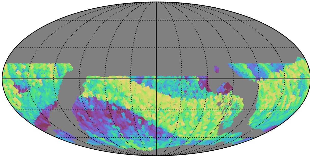
noroll_mjdp0_v3.4_10yrs WFD z band: Max airmass
