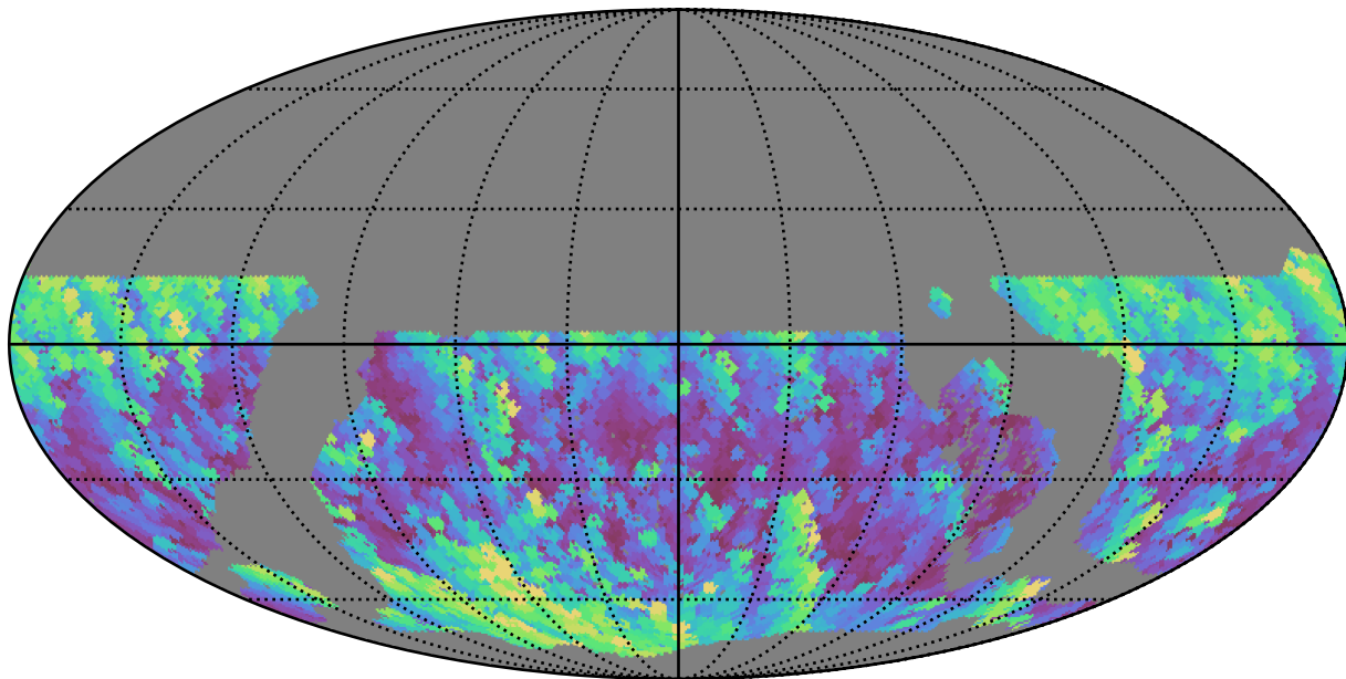
noroll_mjdp0_v3.4_10yrs WFD y band: Max airmass
