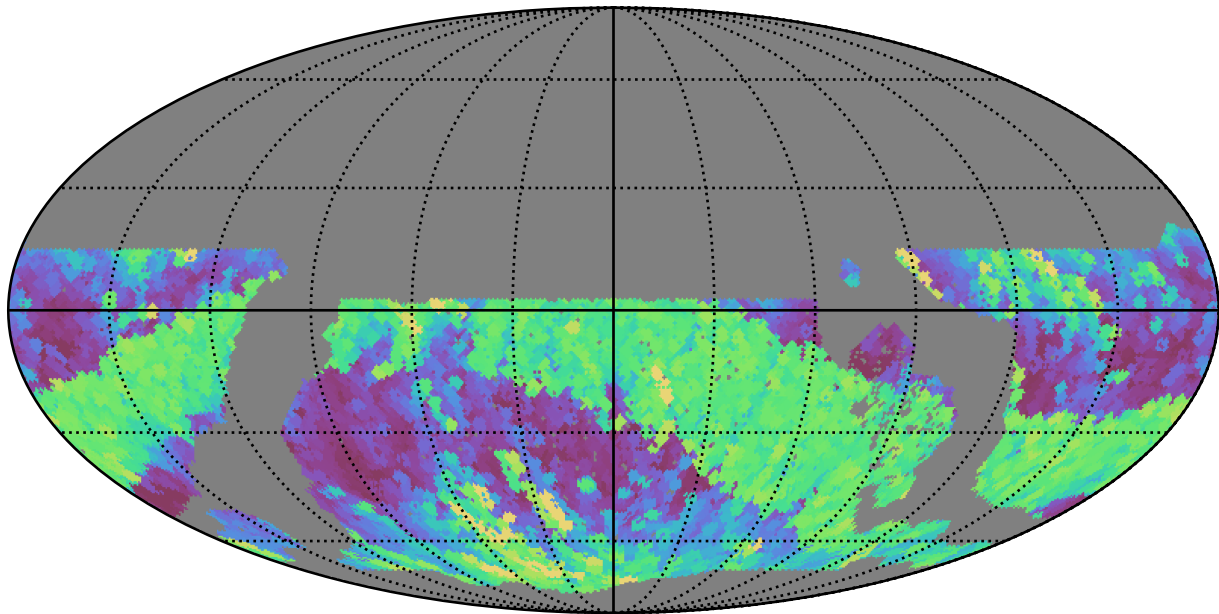
noroll_mjdp0_v3.4_10yrs WFD r band: Max airmass
