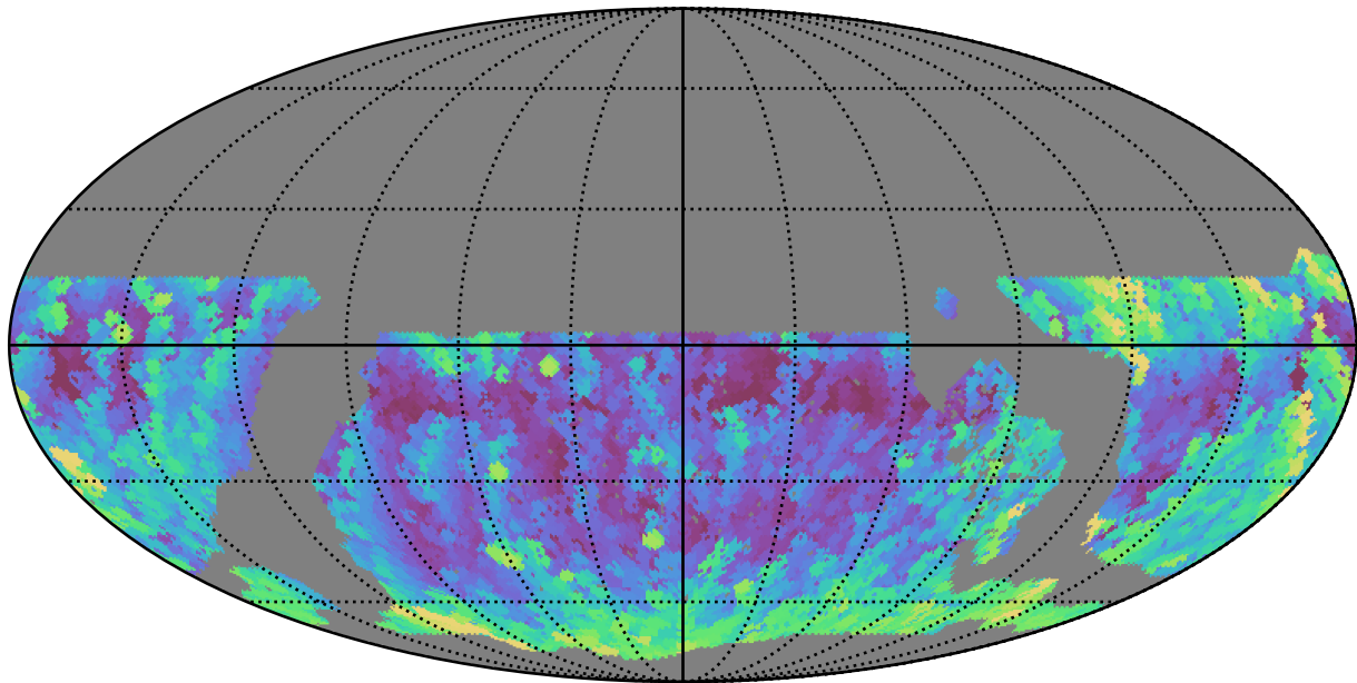
noroll_mjdp0_v3.4_10yrs WFD g band: Max airmass
