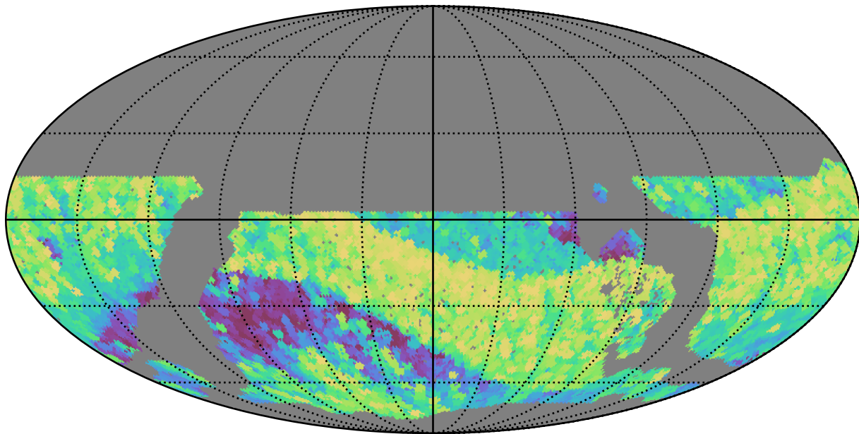
noroll_mjdp0_v3.4_10yrs WFD all bands: Max airmass
