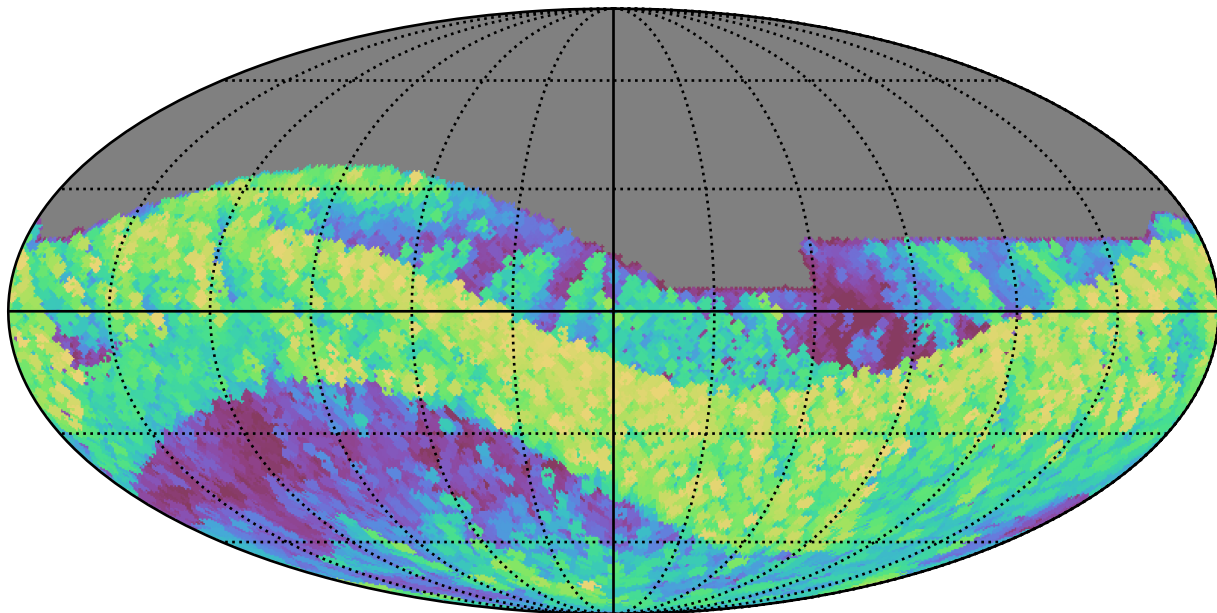
noroll_mjdp0_v3.4_10yrs All sky z band: Max airmass
