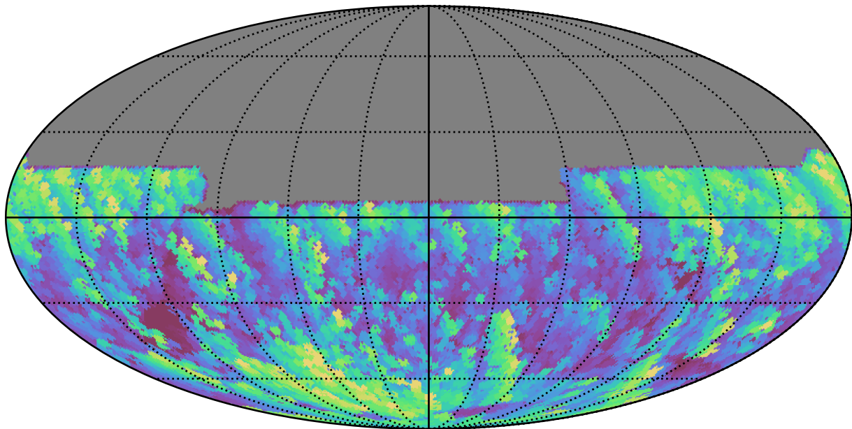
noroll_mjdp0_v3.4_10yrs All sky y band: Max airmass
