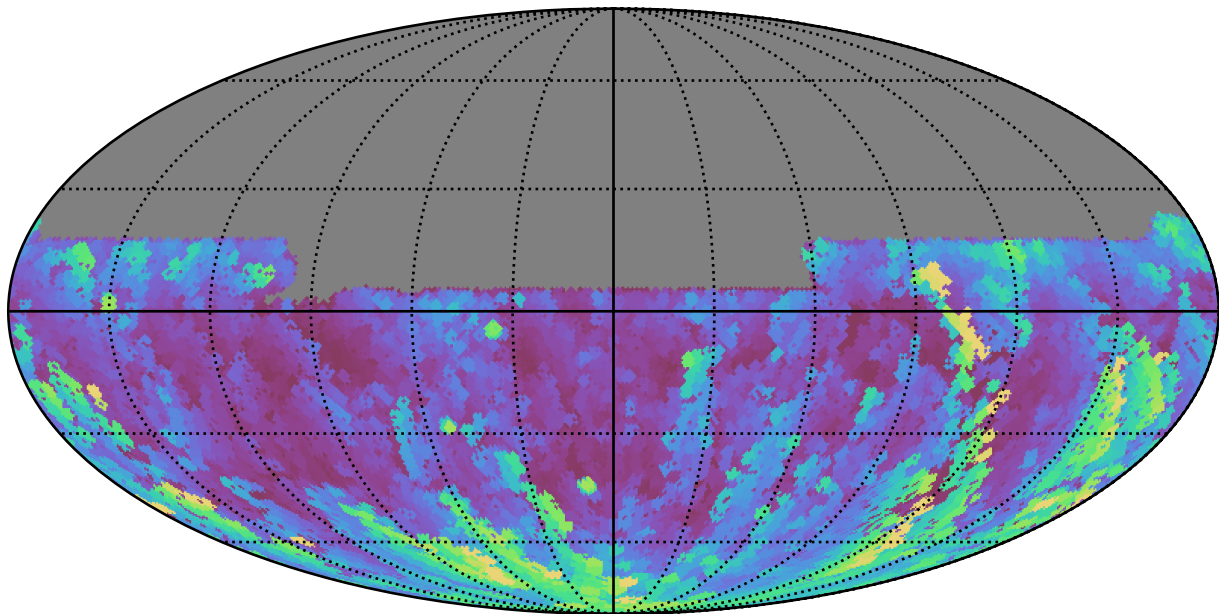
noroll_mjdp0_v3.4_10yrs All sky u band: Max airmass
