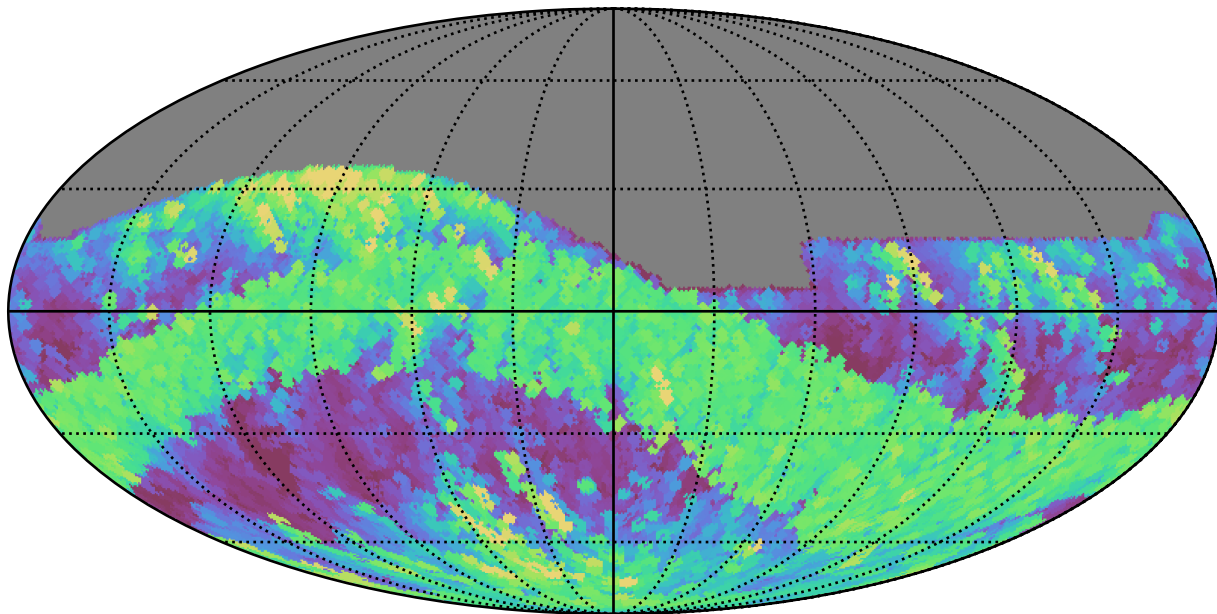
noroll_mjdp0_v3.4_10yrs All sky r band: Max airmass
