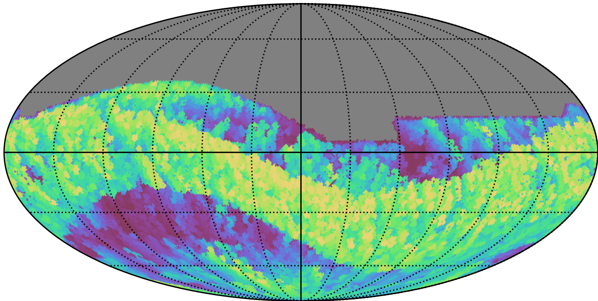
noroll_mjdp0_v3.4_10yrs All sky i band: Max airmass
