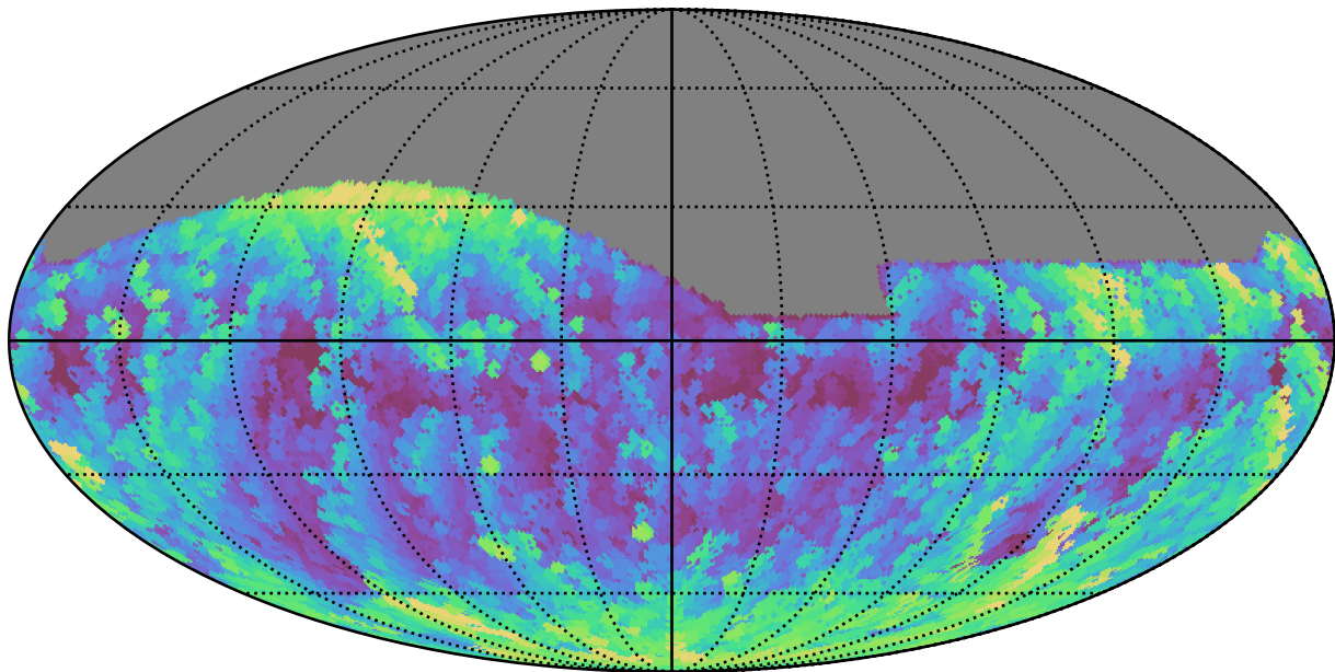
noroll_mjdp0_v3.4_10yrs All sky g band: Max airmass
