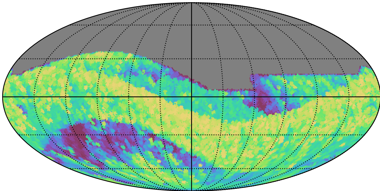
noroll_mjdp0_v3.4_10yrs All sky all bands: Max airmass
