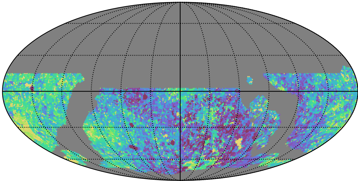
noroll_mjdp0_v3.4_10yrs WFD z band: Max Inter-Night Gap
