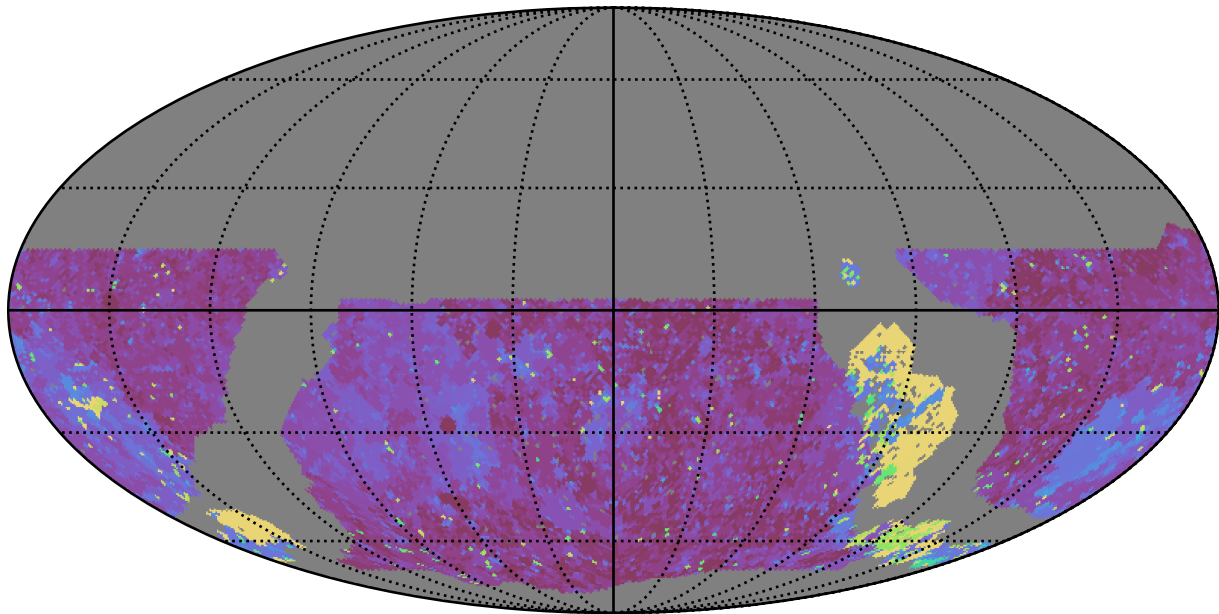
noroll_mjdp0_v3.4_10yrs WFD u band: Max Inter-Night Gap
