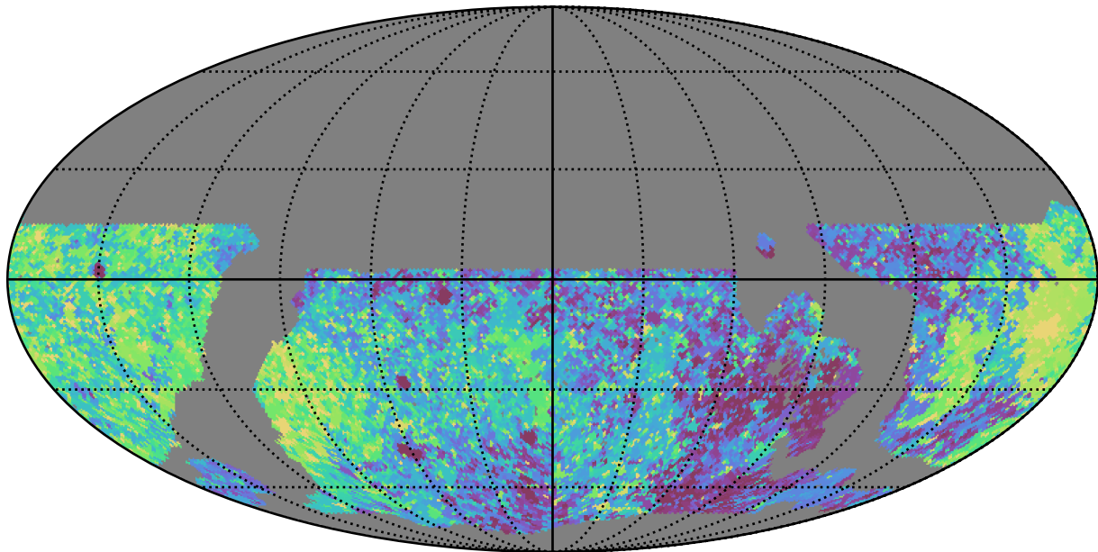
noroll_mjdp0_v3.4_10yrs WFD r band: Max Inter-Night Gap
