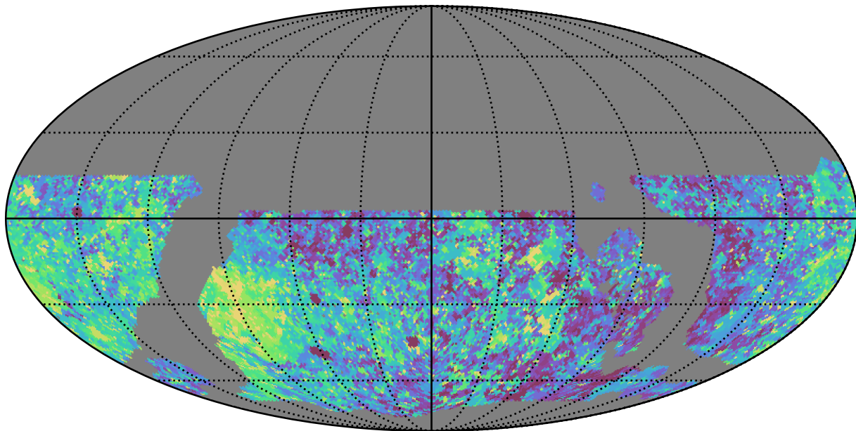
noroll_mjdp0_v3.4_10yrs WFD i band: Max Inter-Night Gap
