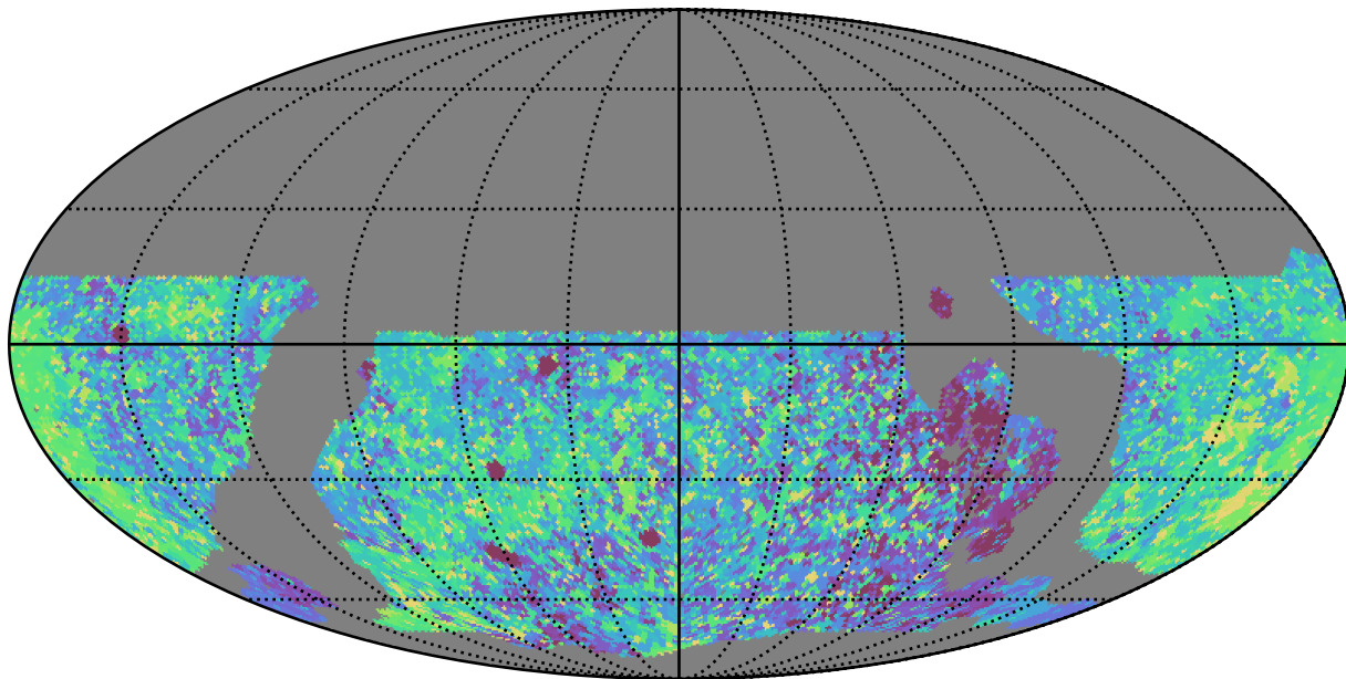
noroll_mjdp0_v3.4_10yrs WFD g band: Max Inter-Night Gap
